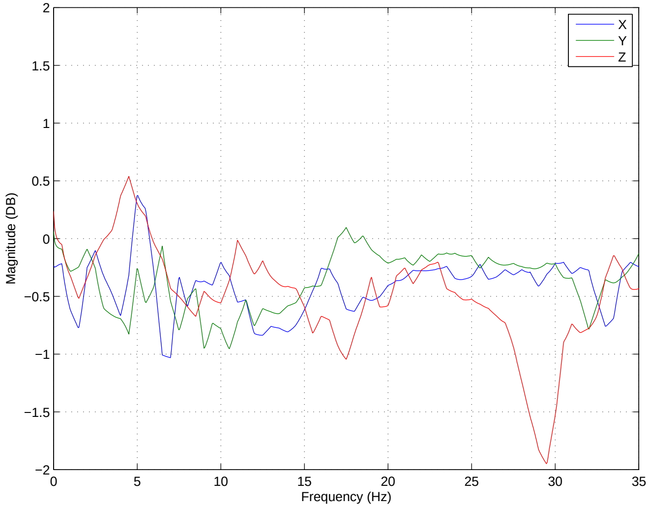
X,Y,Z Axis Tuning Transfer Functions – 600 gal
