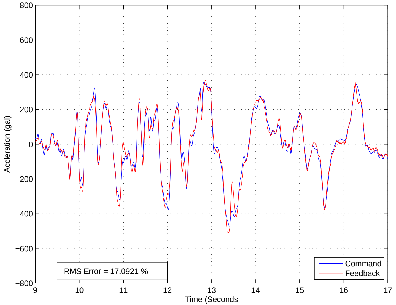
JR Takatori X-Axis Acceleration – 70% Gain
