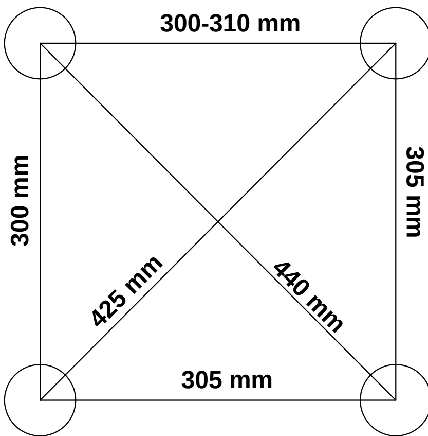
Actuator Mounting shown in Figure 8
