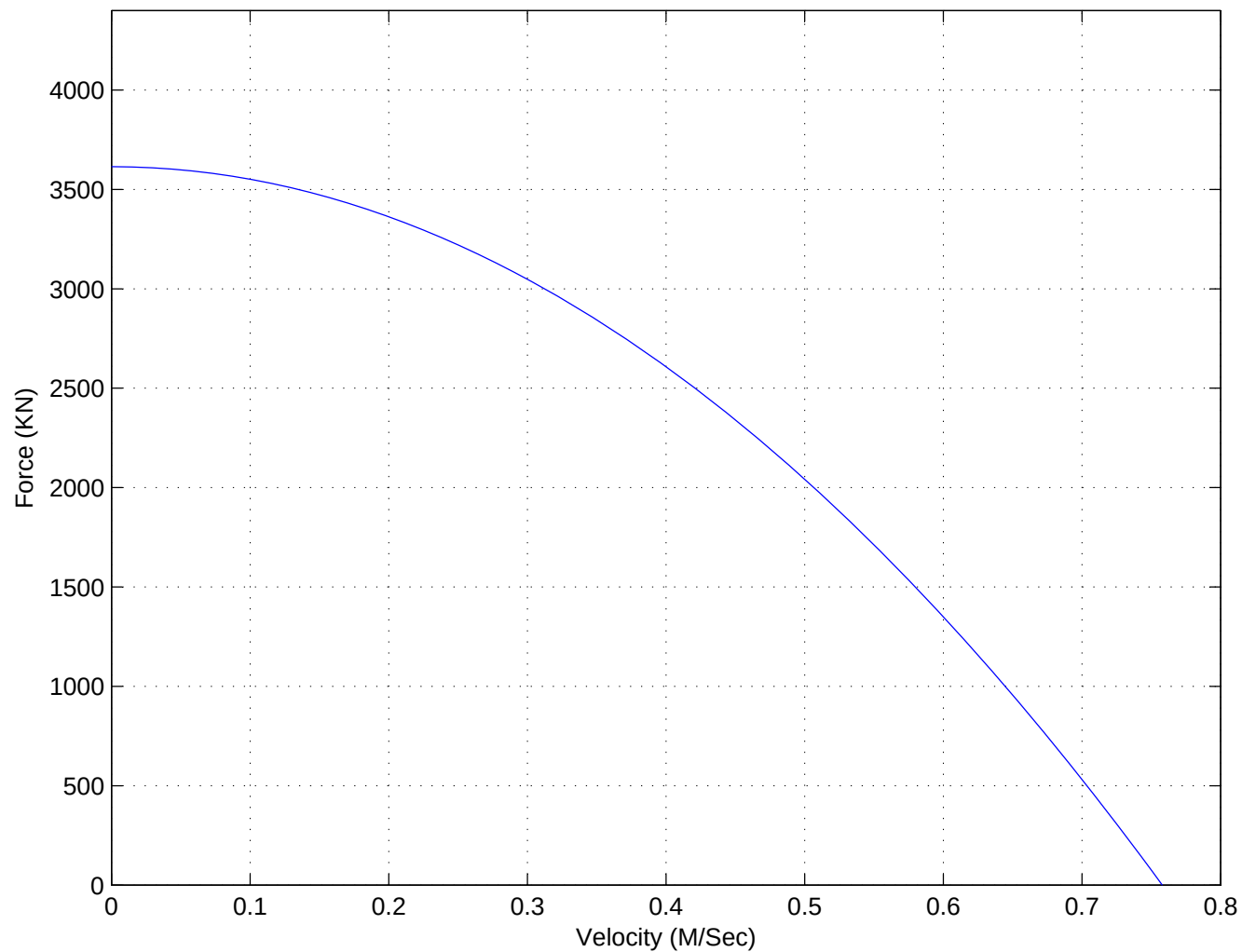
DTS2500 Force-Velocity Curve -230 bar
