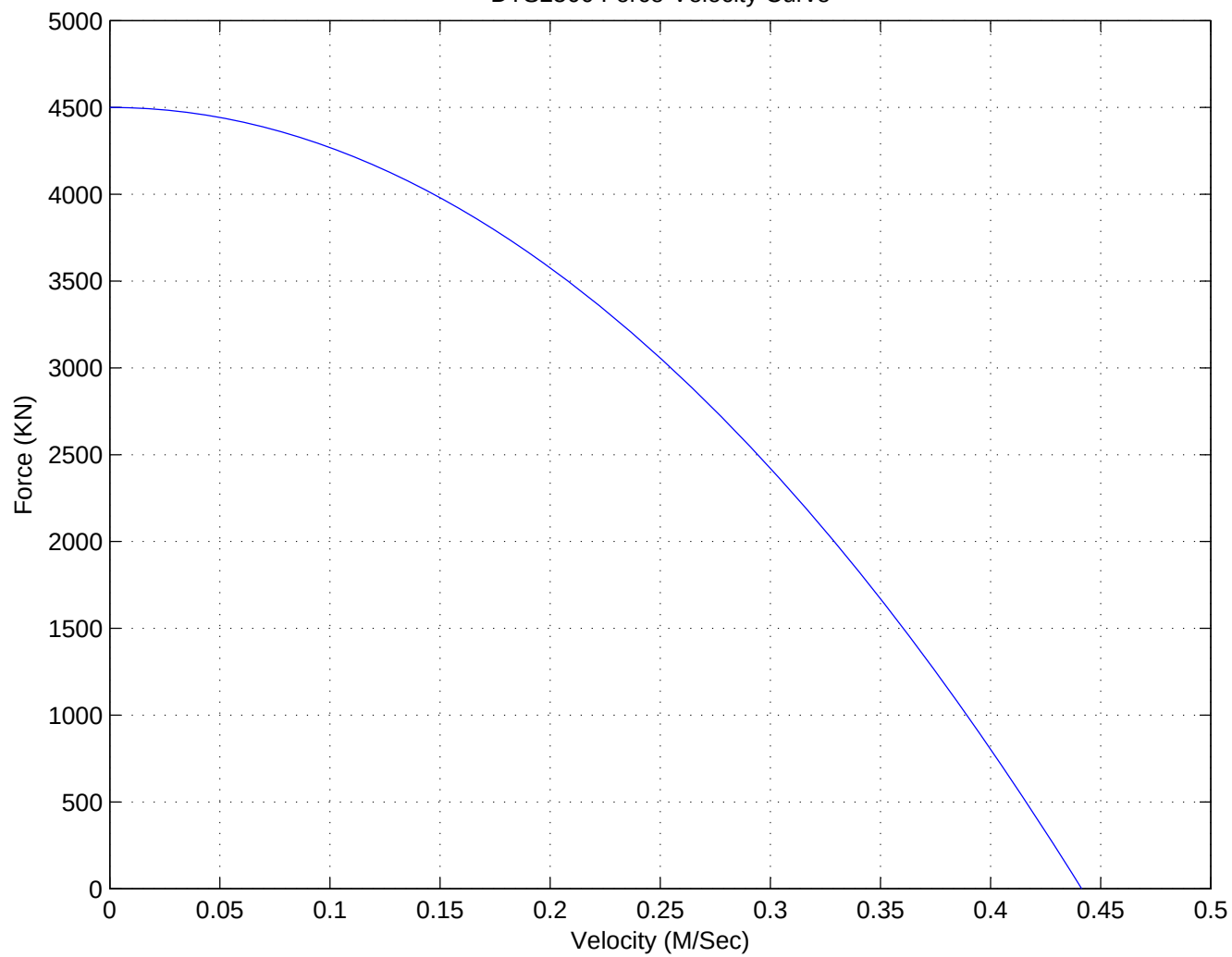
DTS2500 Force-Velocity Curve
