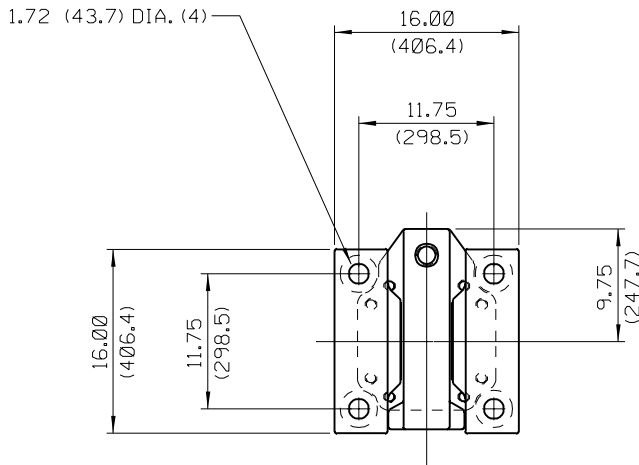
SWIVEL MOUNTING TYP BOTH ENDS
